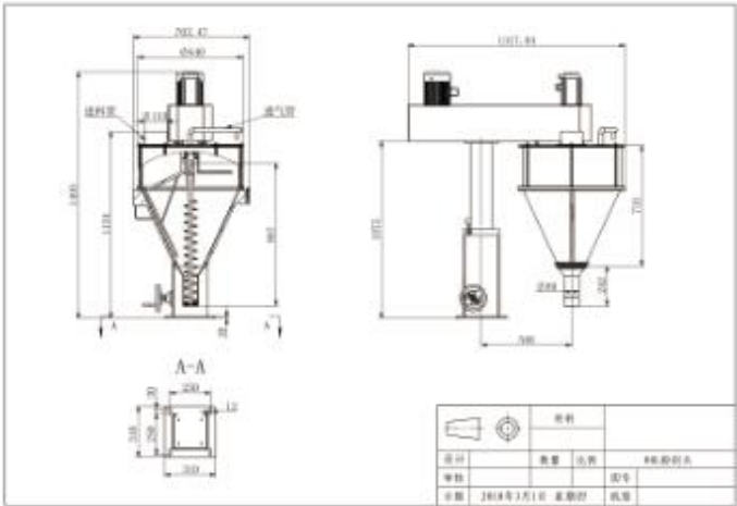
80L螺杆计量机 80L Screw Metering Machine
