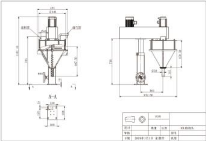
30L螺杆计量机 30L Screw Metering Machine
