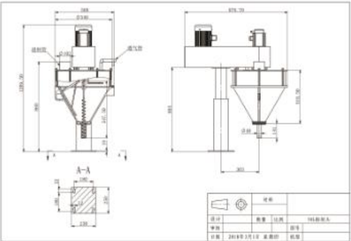
50L螺杆计量机 50L Screw Metering Machine
